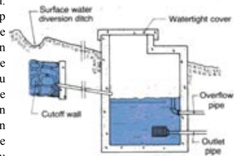
Figure 1a. Cut-away view of a concentrated spring.
